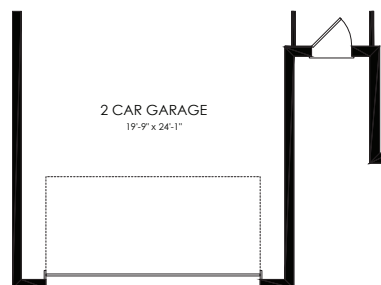
4' Garage Extension
