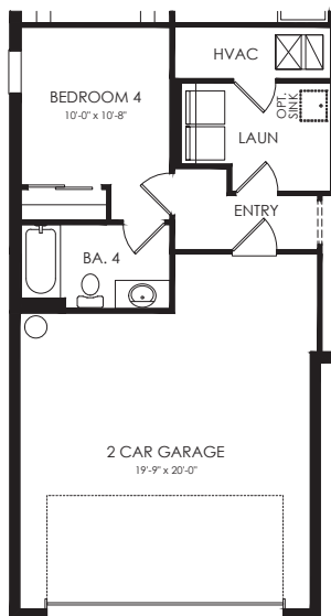
Bath 4 w/ 4' Garage Extension Add 210 SF
